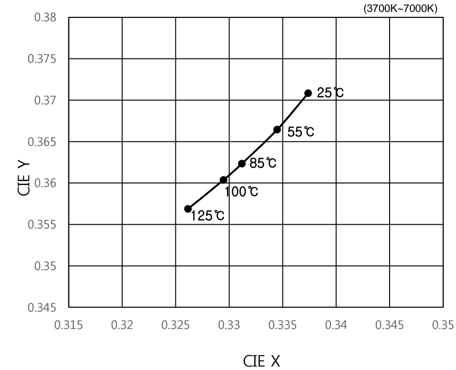
Fig 8. Chromaticity Coordinate vs. Junction Temperature, I_F=120\text{mA}
