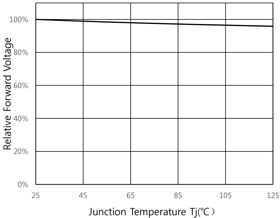
Fig 7. Junction Temperature vs. Relative Forward Voltage, I_F=120\text{mA}
