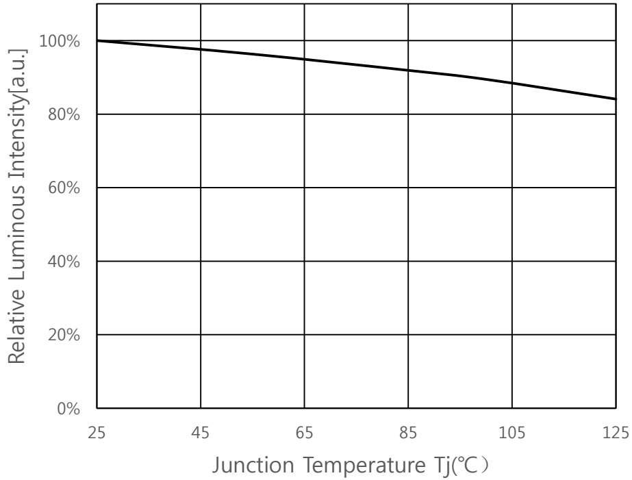
Fig 6. Junction Temperature vs. Relative Luminous Intensity, I_F=120\text{mA}
