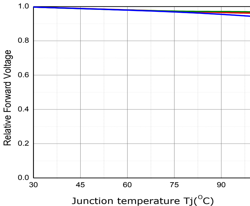
Fig 6. Junction Temperature vs. Relative Forward Voltage, I_F=20\text{mA}
