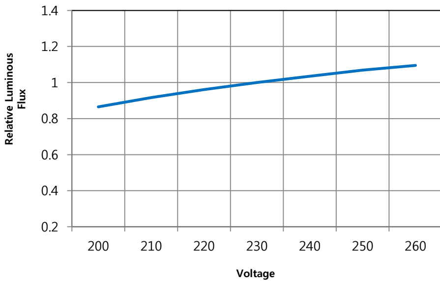
Fig 7. Relative Luminous Flux vs. Voltage, T_a=25^{\circ}\text{C} , 230V
