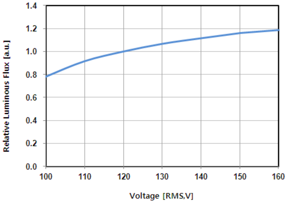
Fig 6. Relative Luminous Flux vs. Voltage, T_a=25^{\circ}\text{C} , 120V
