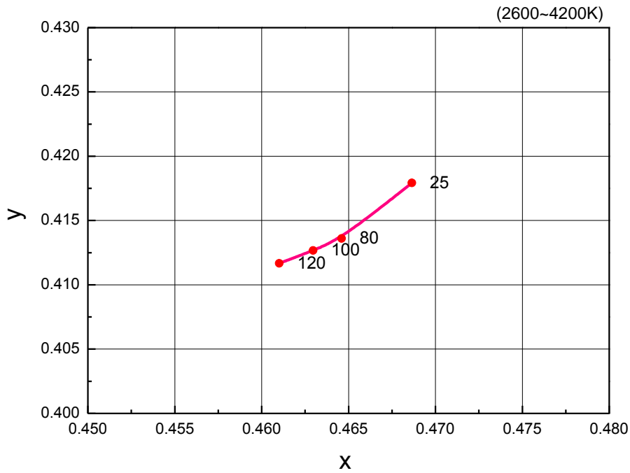
Fig 8. Chromaticity Coordinate vs. Junction Temperature, I_F=50mA
