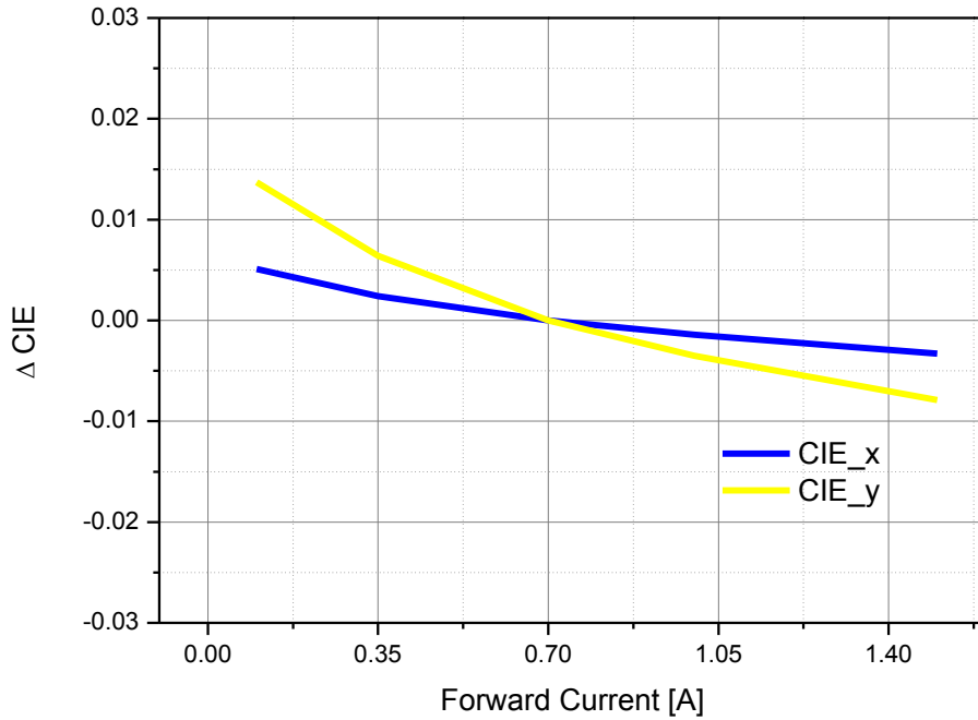
Forward Current vs \Delta CIE , T_a=25^\circ C
